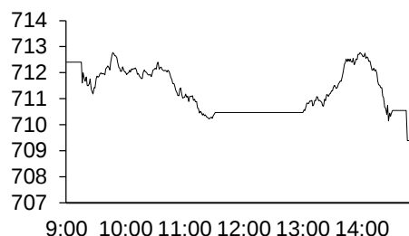
VN-Index Intraday
