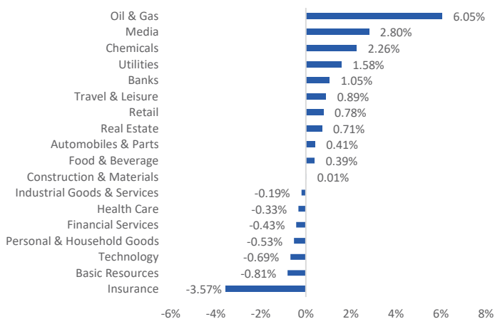
Figure 1 Sectors performance
