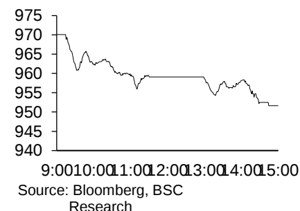
HSX-Index Intraday
