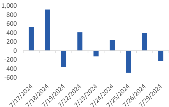
Figure 4 Foreign transactions
